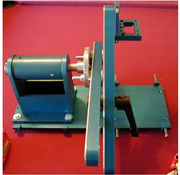
Cardan Fixtures mounted on the ADVANCED Maintenance Solutions Alignment Simulator
